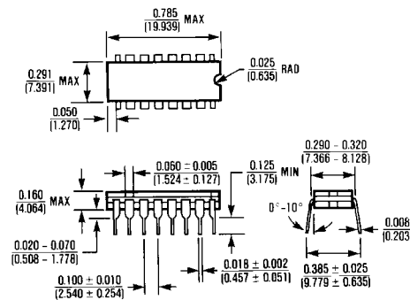
16 Lead CERP
